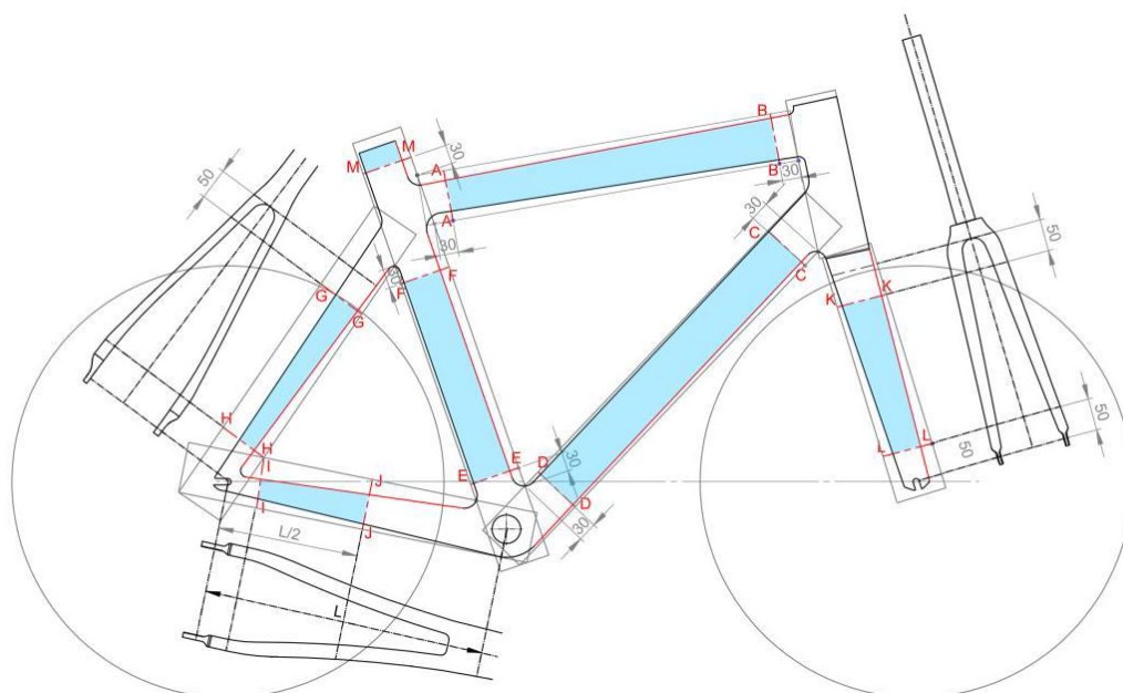
Figure 14: Illustration of the areas of the frame and forks subject to the rule of minimum and maximum dimension for the tubes, for road and cyclo-cross models
