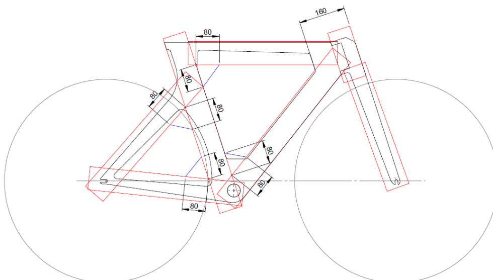
Figure 24: Illustration of compensation triangles
