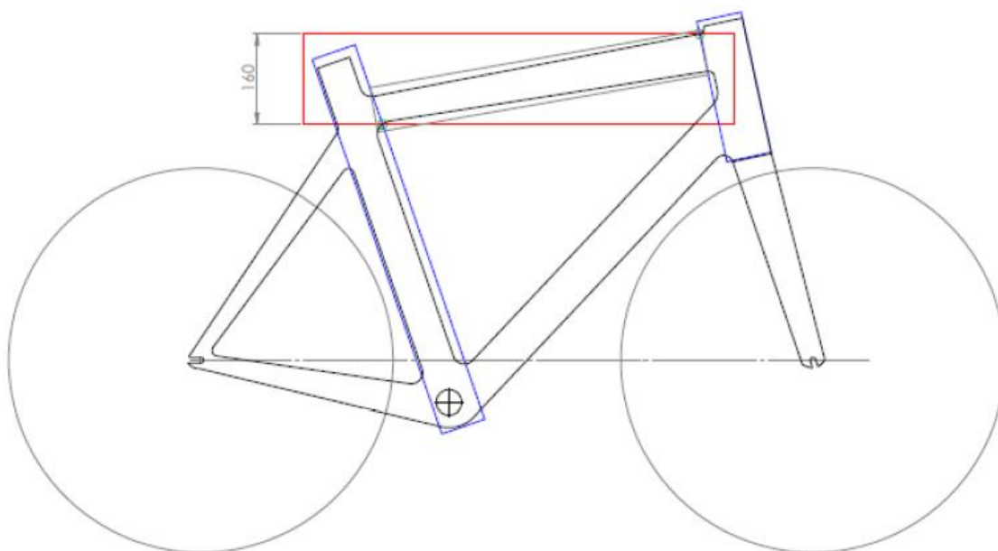
Figure 15: Illustration of maximum allowed sloping top tube
