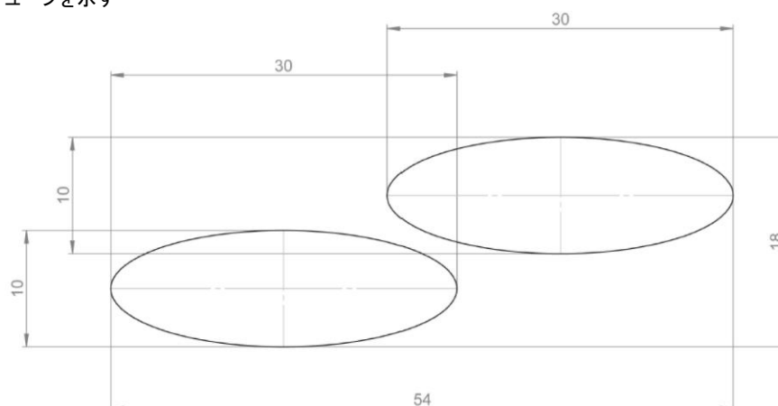
Figure 26: Example of a compliant section of an element formed by two tubes (minimum section of 1 cm applied to the fork, seat stays or chain stays)
