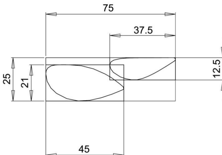
Figure 28: Example of a compliant section of an element formed by two tubes (minimum section of 1 cm applied to the fork, seat stays or chain stays)
