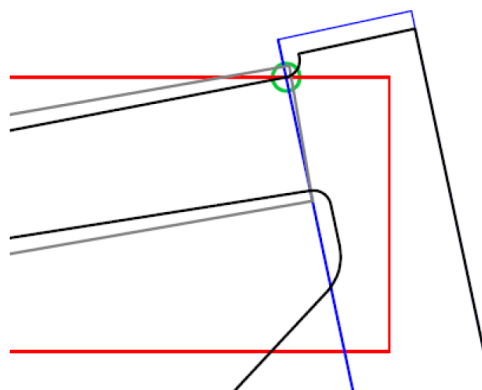
Figure 17: Highest point (circled in green) that must be contained within the 16 cm-high horizontal box
