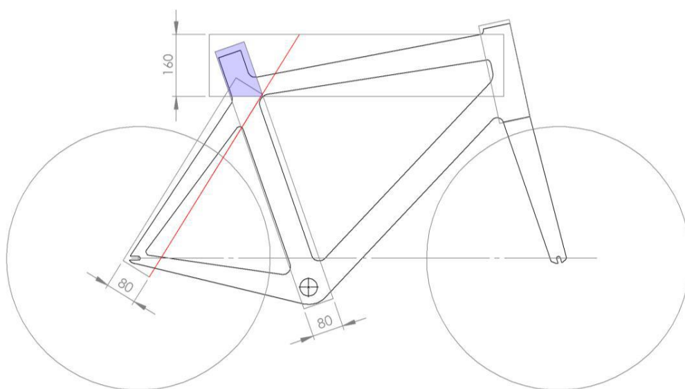
Figure 25: Illustration of the rule on the inclination of seat stays
