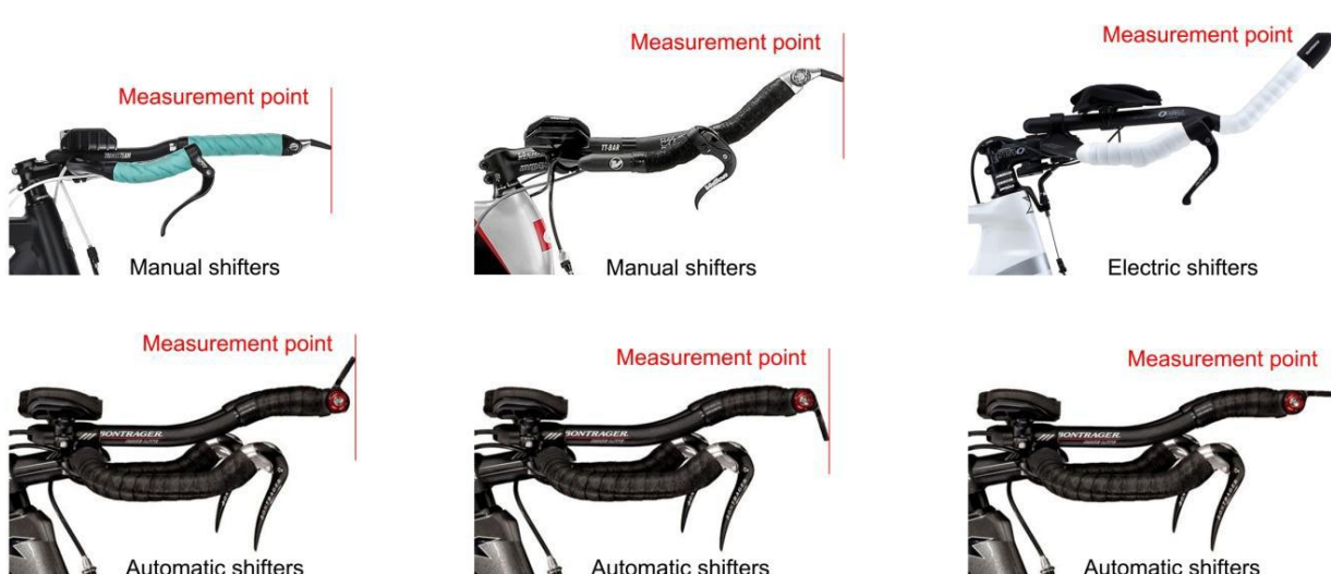
Figure 40: Points of measurement for the horizontal distance from the bottom bracket axle
