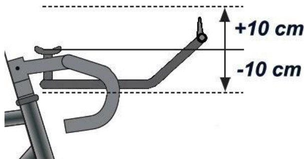
Figure 41: Illustration of the vertical limits of the handlebars extensions including accessories
