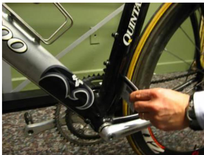
Figure 53: Insertion of a credit card between the wheel and frame to check that a fairing is not present
