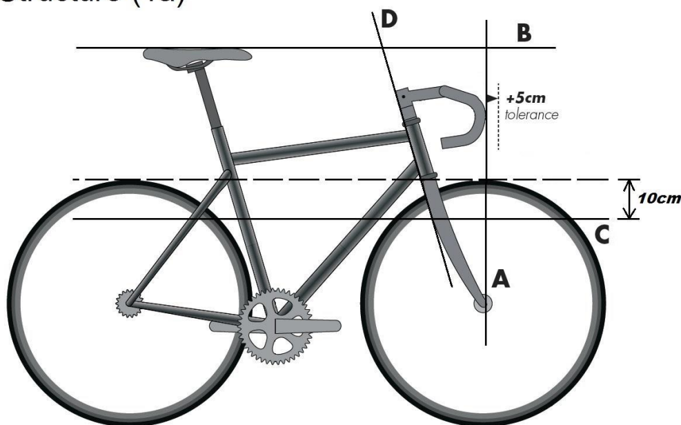
Figure 39: Illustration of the box, marked out by lines A, B, C and D, within which the handlebars must be fully contained.
