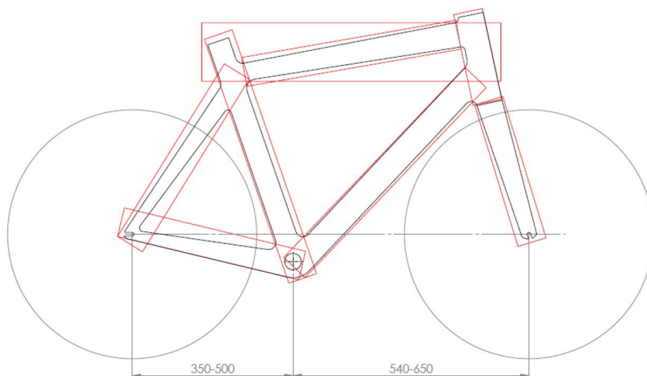
Figure 5: Illustration of the minimum and maximum distances between the bottom bracket and front and rear wheel axles 図 5: ボトム・ブラケットと前車軸と後車軸間の最小/最大距離の説明
