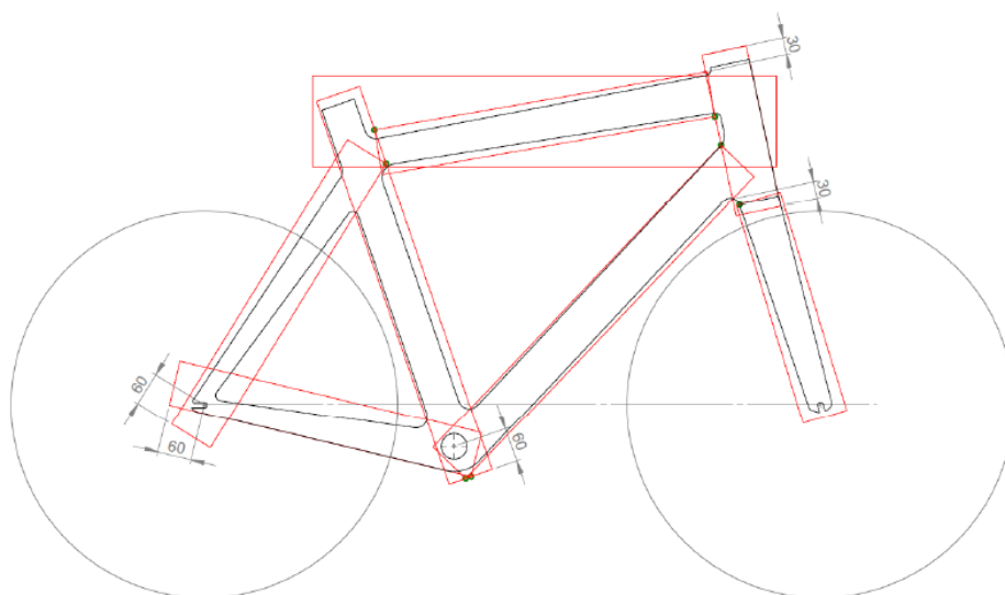
Figure 12: Illustration of the template showing the start and finish points of the 8 cm boxes for each element
