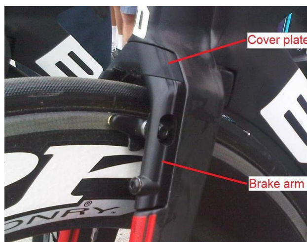
Figure 48: Brake integrated with the fork and fitted with a cover
