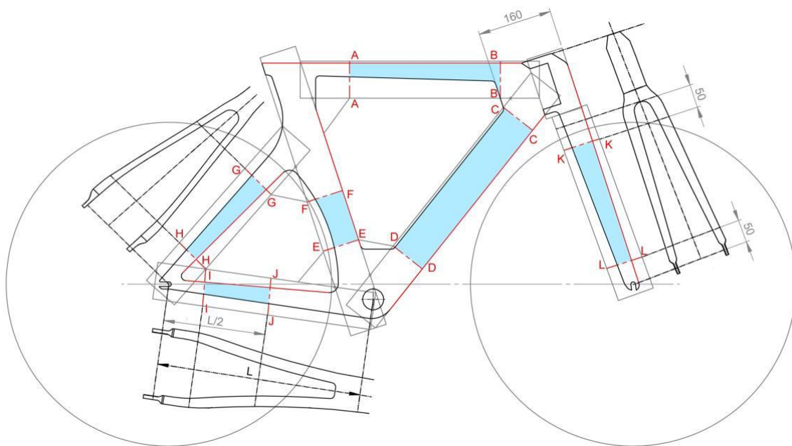
Figure 21: Illustration of the sections of the frame and forks subject to the rule of minimum and maximum dimension for the tubes, for time trial and track models
