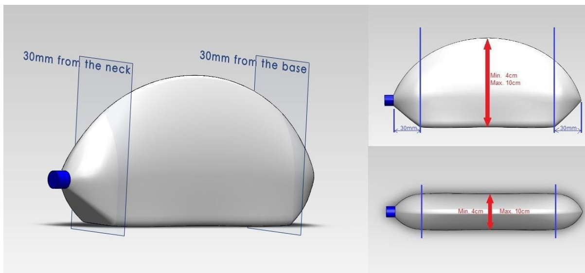
Figure 56: Illustration of the areas of a bottle where the dimensions are subject to regulations
