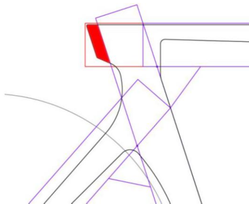
Figure 25: Illustration of the unauthorised extension of the top tube box behind the seat tube
