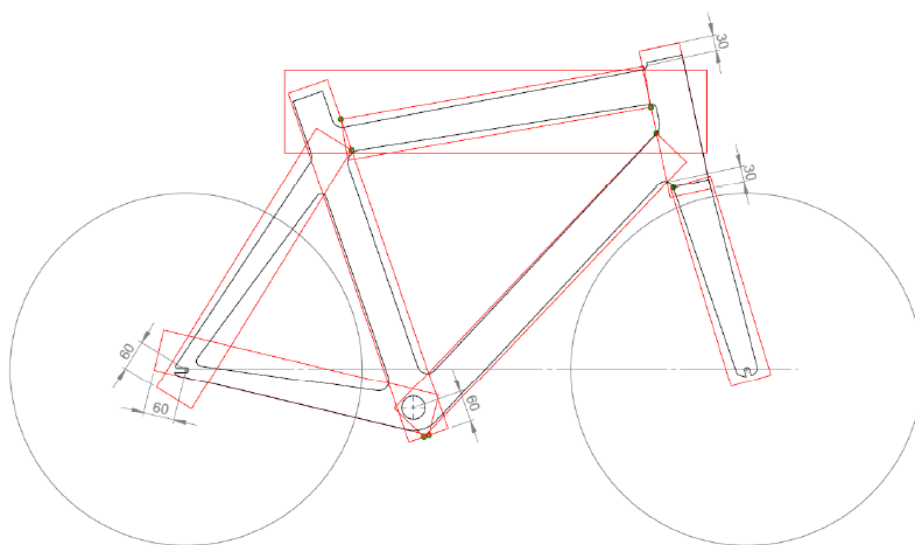
Figure 14: Illustration of the template showing the start and finish points of the 8 cm boxes for each element
