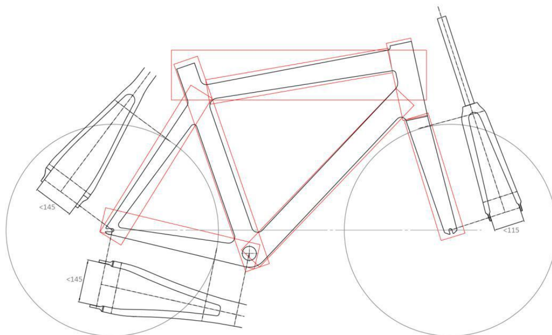
Figure 8: Illustration of the maximum distances between the fork drop-outs and rear drop-outs 図8: 前エンド幅と後ろエンド幅の最大距離の説明
