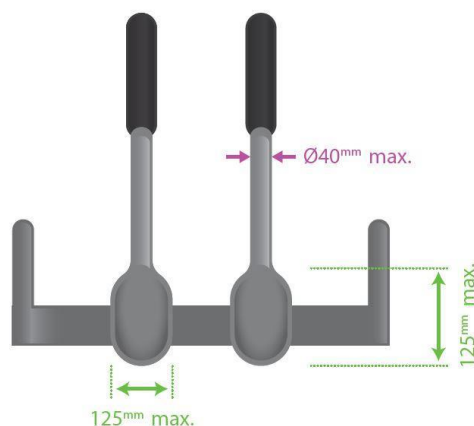
Figure 42: Illustration of the case of the maximal length and width of elbow rests and the maximal width and height of extensions
