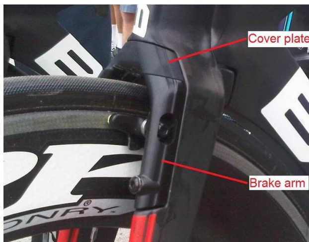
Figure 50: Brake integrated with the fork and fitted with a cover
