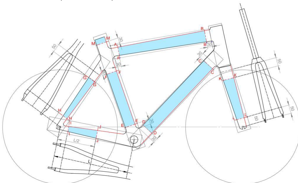
Figure 16: Illustration of the areas of the frame and forks subject to the rule of minimum and maximum dimension for the tubes, for road and cyclo-cross models
