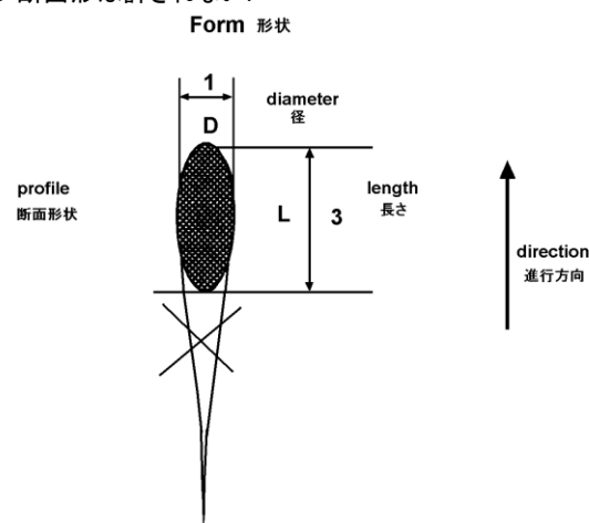
Figure 53: Illustration of the 3:1 rule restricting the fuselage form of elements
