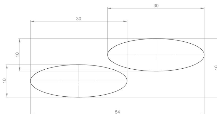
Figure 28: Example of a compliant section of an element formed by two tubes (minimum section of 1 cm applied to the fork, seat stays or chain stays)
