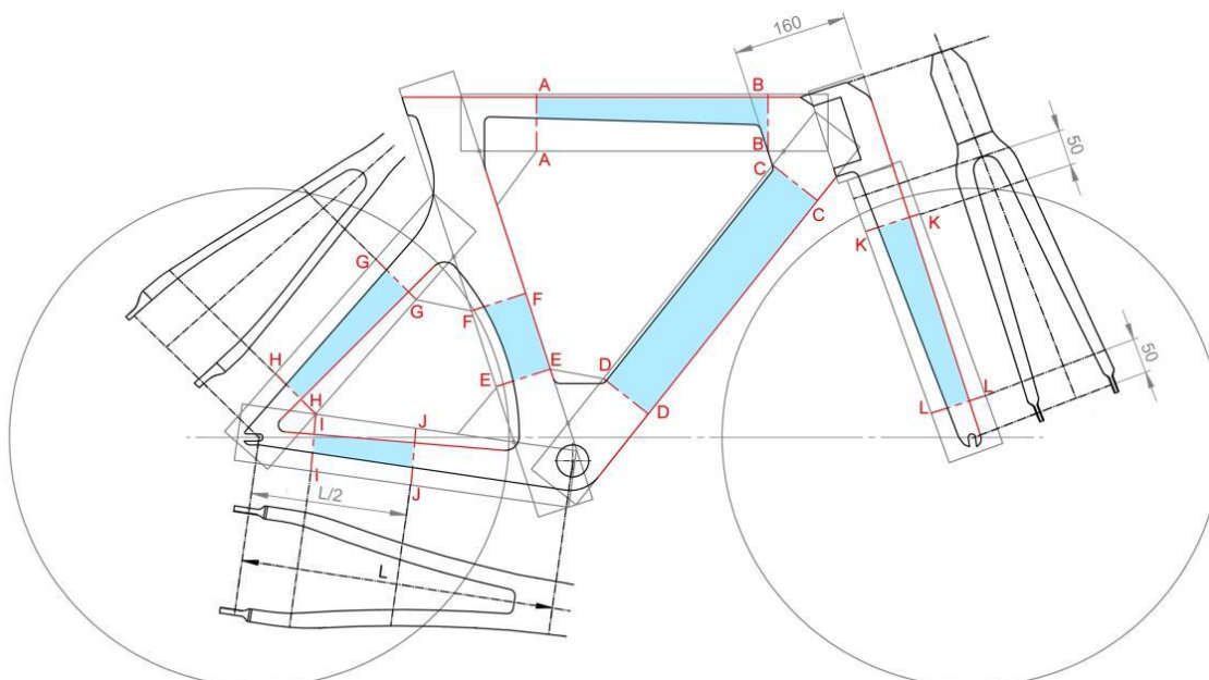
Figure 23: Illustration of the sections of the frame and forks subject to the rule of minimum and maximum dimension for the tubes, for time trial and track models
