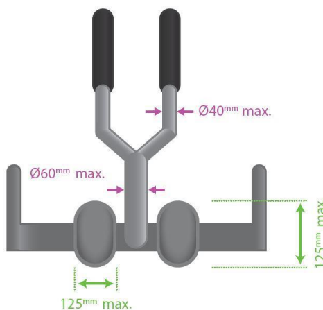
Figure 43: Illustration of the case when both extensions are joined by part
