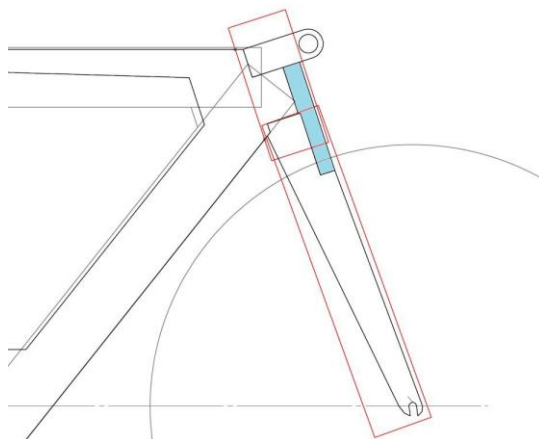
Figure 52: Illustration of a cover that fits over the brake and extends to the stem
