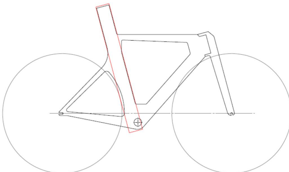
Figure 22: Illustration of the extension of the seat tube
