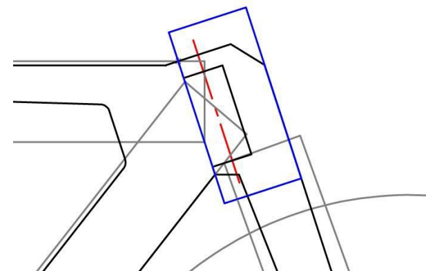
Figure 38: Illustration of the positioning of the axis of the head tube within the head tube box
