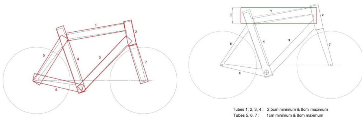
Figure 13: General illustration of the shape and positioning of the 8 cm boxes
