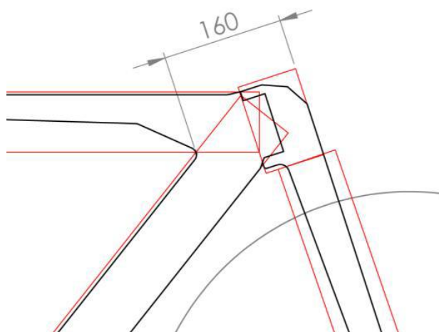
Figure 35: Illustration of the limit case
