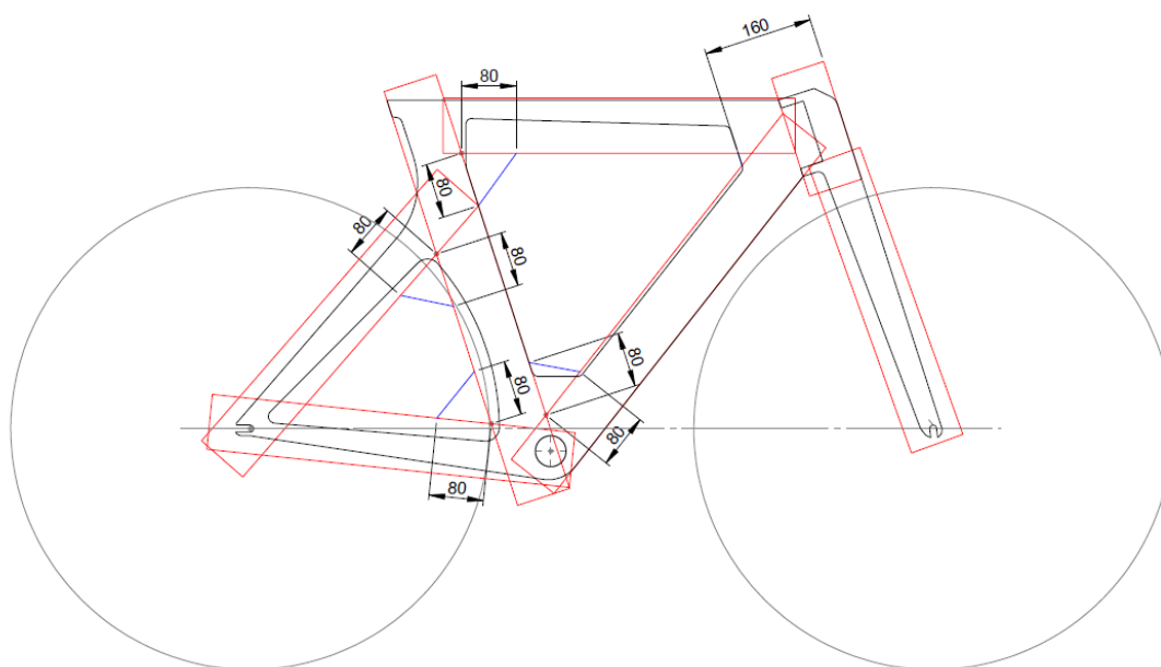
Figure 26: Illustration of compensation triangles
