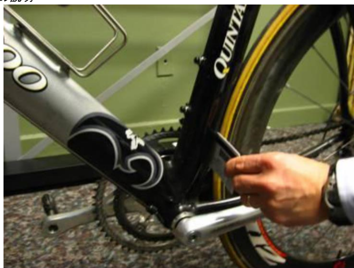
Figure 55: Insertion of a credit card between the wheel and frame to check that a fairing is not present
