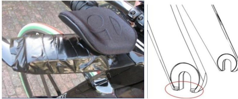
Figure 1: Examples of the prohibited modification of equipment (addition of tape, filing off fork drop-out safety lugs) 図 1: 禁じられる機材修正の例(テープの追加, フォークの安全ラグの削り落とし)
