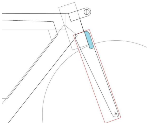
Figure 51: Illustration of a cover that fits over the brake only
