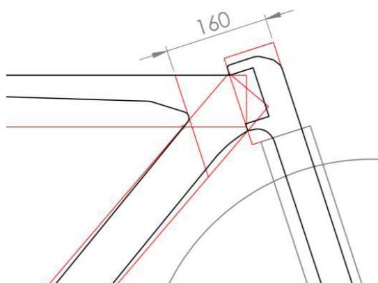
Figure 34: Illustration of the maximum distance of 16 cm for a small frame size (B)
