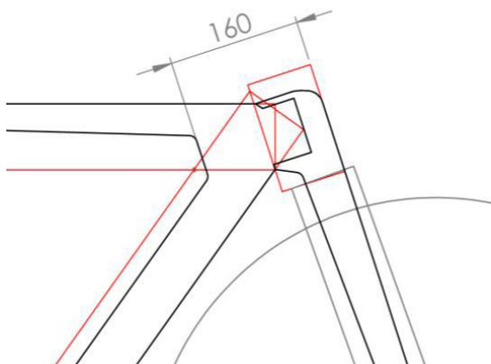
Figure 33: Illustration of the maximum distance of 16 cm for a small frame size (A)
