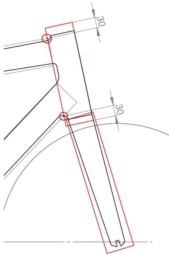
Figure 37: Illustration of the position of the boxes for a fork using a traditional internal steerer
