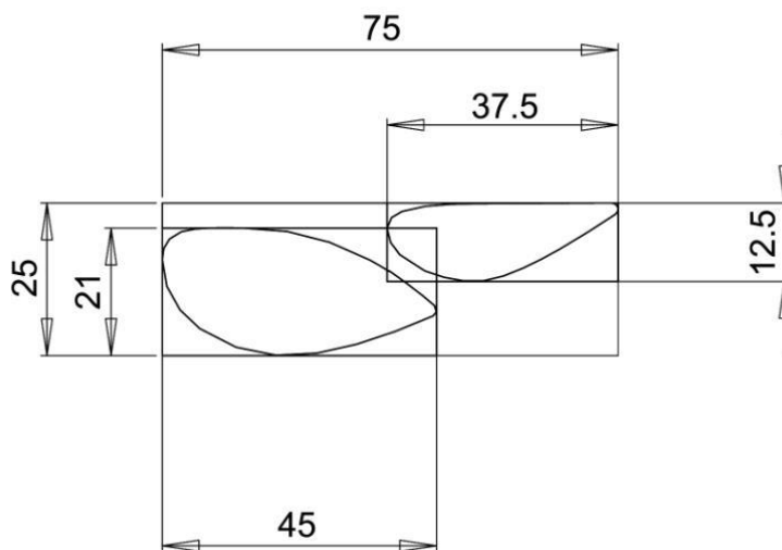
Figure 30: Example of a compliant section of an element formed by two tubes (minimum section of 1 cm applied to the fork, seat stays or chain stays)
