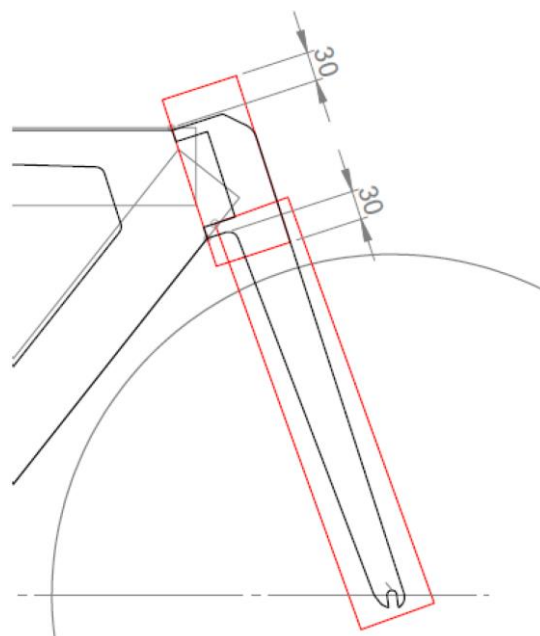
Figure 39: Illustration of the position of the boxes for offset forks
