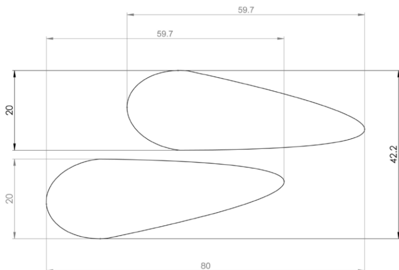
Figure 29: Example of a compliant section of an element formed by two tubes (minimum section of 1 cm applied to the fork, seat stays or chain stays)
