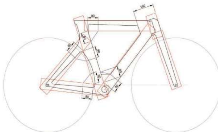
Position of compensation triangle Shape (3) 補強三角形の位置 形状(3)
